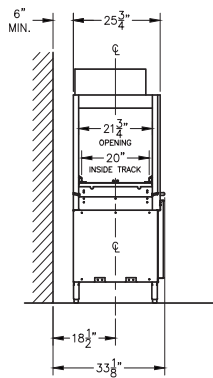
End View
